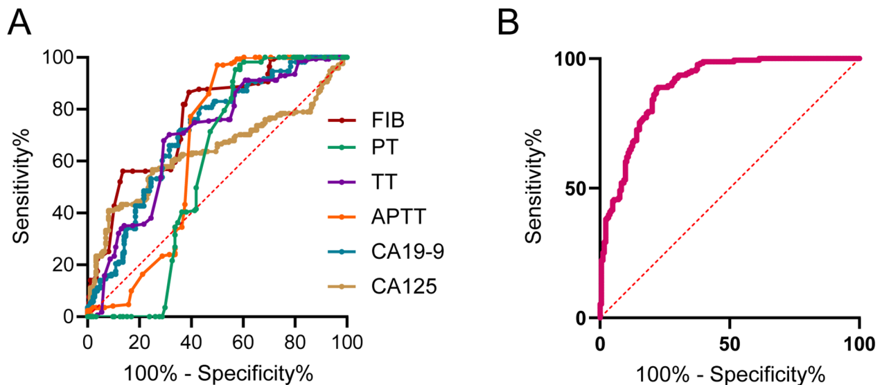
Fig. 3 Receiver operating characteristic curves of CA125, CA199, coagulation factors and the combined marker for the diagnosis of endometriomas with stage IV. a , The ROC analysis of CA125, CA199 and coagulation factors for the diagnosis of endometriomas with stage IV. b , The ROC analysis of combined marker for the diagnosis of endometriomas with stage IV. ROC, receiver operating characteristic; APTT, activated partial thromboplastin time; TT, thrombin time; PT, prothrombin time; FIB, fibrinogen; NLR, neutrophil-to-lymphocyte ratio
